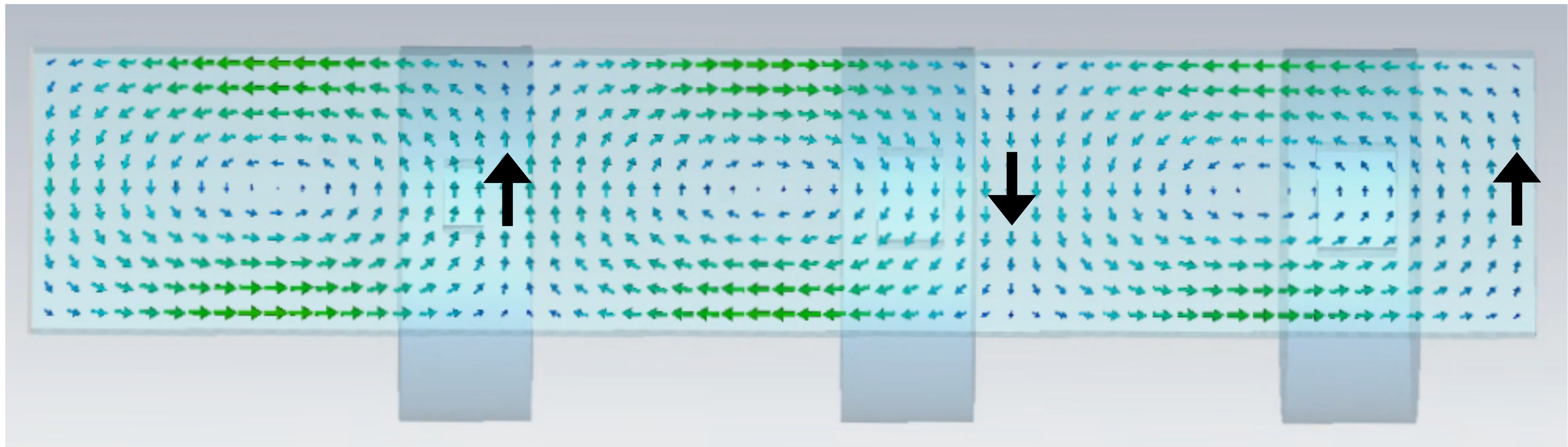
View of magnetic fields in a waveguide driven at 805 MHz
